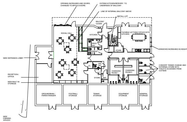
GROUND FLOOR 1:100
