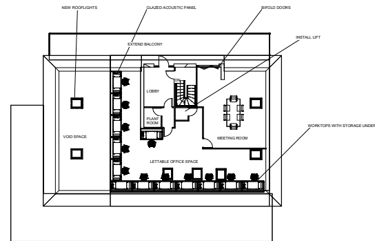
FIRST FLOOR 1:100
