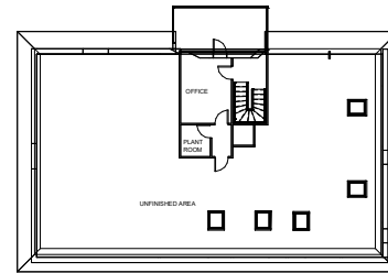
FIRST FLOOR 1:100
